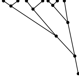
FIGURE 1. Branching geodesics as described in §1.1.2.
