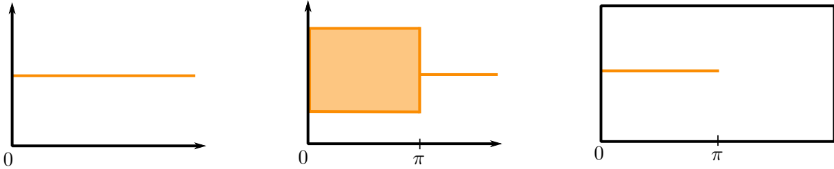
FIGURE 4. (Left to Right): The output dendrograms of the nonreciprocal and reciprocal clustering methods on \vec{\mathbb{S}}^1 , and a persistence barcode representing the diagram \{(0, \pi)\} . See Theorems 26, 27, and 28.
