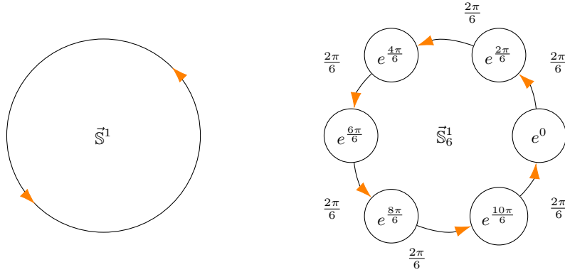
FIGURE 3. The directed circle \vec{\mathbb{S}}^1 and a directed circle on 6 nodes \vec{\mathbb{S}}_6^1 . By the results in [CM17a], we have d_{\mathcal{N}}(\vec{\mathbb{S}}^1, \vec{\mathbb{S}}_6^1) \leq \frac{\pi}{3} . By Theorem 25, we have \text{Dgm}_1^{\mathcal{D}}(\vec{\mathbb{S}}_6^1) = \{(\frac{\pi}{3}, \pi) \in \mathbb{R}^2\} .
