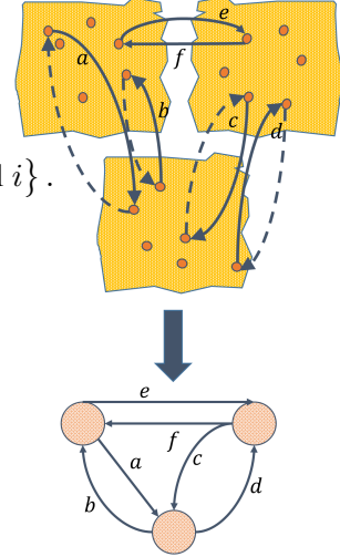
FIGURE 2. Networks arising from disconnected networks
