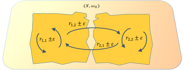
FIGURE 1. Elements of an \epsilon -system on X , as described in Definition 4.
