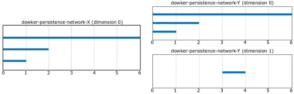
FIGURE 9. Dowker persistence barcodes of networks (X, \omega_X) and (Y, \omega_Y) from Figure 8.
