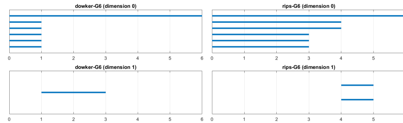
FIGURE 3. The first column contains illustrations of cycle networks G_3, G_4, G_5 and G_6 . The second column contains the corresponding Dowker persistence barcodes, in dimensions 0 and 1. Note that the persistent intervals in the 1-dimensional barcodes agree with the result in Theorem 33. The third column contains the Rips persistence barcodes of each of the cycle networks. Note that for n = 3, 4 , there are no persistent intervals in dimension 1. On the other hand, for n = 6 , there are two persistent intervals in dimension 1.
