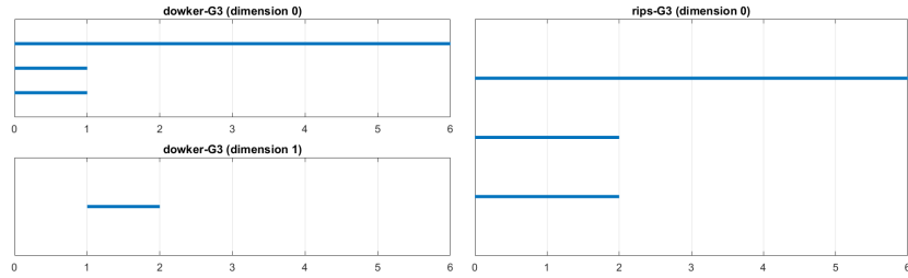
The cycle network G_3
