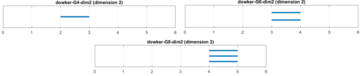
FIGURE 7. Sample 2-dimensional Dowker persistence barcodes for cycle networks G_4, G_6, G_8 . In our experiments, 2-dimensional Dowker persistence barcodes for G_n were always empty for n odd.
