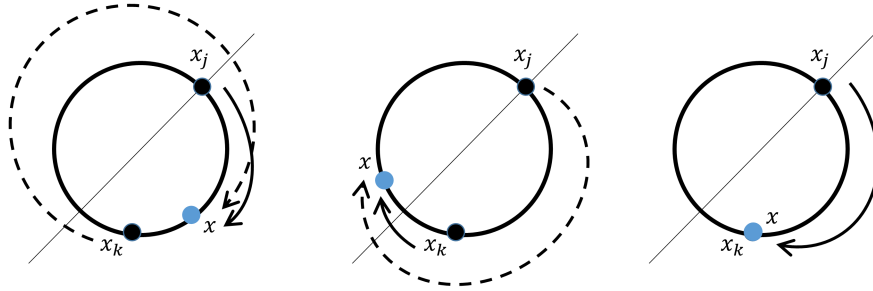
FIGURE 5. Three possible locations for a \delta -sink x of a simplex [x_j, x_k] , assuming that \omega_{G_n}(x_j, x_k) \leq n/2 . For the figure on the left, note that \omega_{G_n}(x_k, x) \geq n/2 \geq \omega_{G_n}(x_j, x_k) . For the figure in the middle, note that \omega_{G_n}(x_j, x) \geq \omega_{G_n}(x_j, x_k) . Finally, for the figure on the right, where x = x_k , note that \omega_{G_n}(x_j, x) = \omega_{G_n}(x_j, x_k) and \omega_{G_n}(x_k, x) = 0 .
