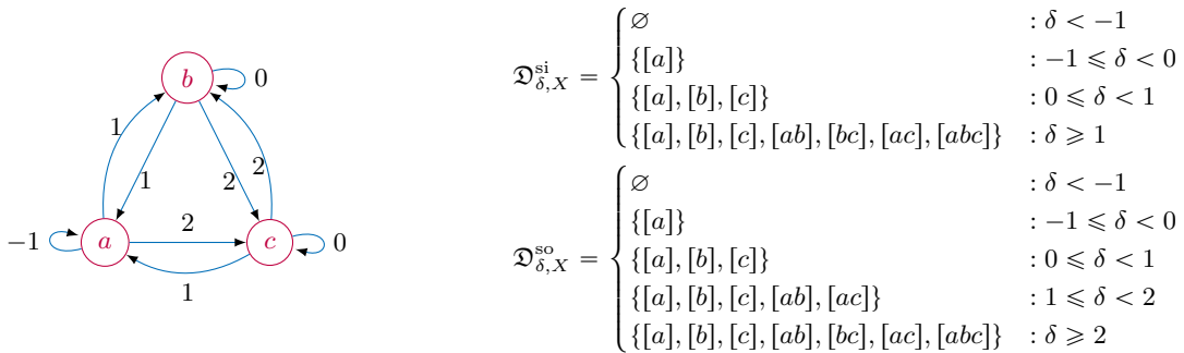
FIGURE 2. Computing the Dowker sink and source complexes of a network (X, \omega_X) . Observe that the sink and source complexes are different in the range 1 \leq \delta < 2 .
