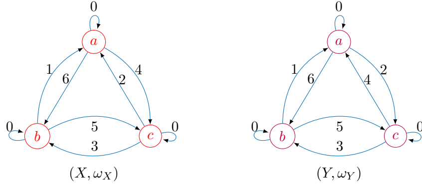
FIGURE 8. (Y, \omega_Y) is the (a, c) -swap of (X, \omega_X) .
