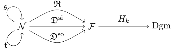
FIGURE 1. A schematic of some of the objects studied in this paper. \mathcal{N} is the collection of all weighted, directed networks (i.e. digraphs with possibly asymmetric real weights). \mathcal{F} is the collection of filtered simplicial complexes. \text{Dgm} is the collection of persistence diagrams. We study the Rips ( \mathfrak{R} ) and Dowker ( \mathfrak{D}^{\text{si}}, \mathfrak{D}^{\text{so}} ) filtrations, each of which takes a network as input and produces a filtered simplicial complex. \mathfrak{s} and \mathfrak{t} denote the network transformations of symmetrization (replacing a pair of weights between two nodes by the maximum weight) and transposition (swapping the weights between pairs of nodes). \mathfrak{R} is insensitive to both \mathfrak{s} and \mathfrak{t} . But \mathfrak{D}^{\text{si}} \circ \mathfrak{t} = \mathfrak{D}^{\text{so}} , \mathfrak{D}^{\text{so}} \circ \mathfrak{s} = \mathfrak{D}^{\text{si}} , and in general, \mathfrak{D}^{\text{si}} and \mathfrak{D}^{\text{so}} are not invariant under \mathfrak{t} (Theorem 43).
