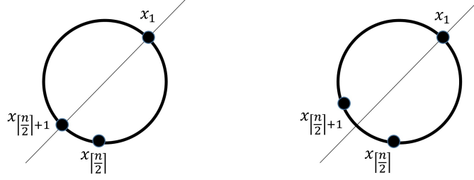
FIGURE 6. Placement of x_{[n/2]} and x_{[n/2]+1} , depending on whether n is even or not.
