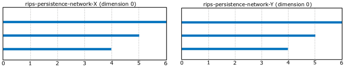
FIGURE 10. Rips persistence barcodes of networks (X, \omega_X) and (Y, \omega_Y) from Figure 8. Note that the Rips diagrams indicate no persistent homology in dimensions higher than 0, in contrast with the Dowker diagrams in Figure 9.
