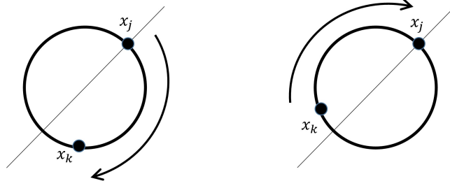
FIGURE 4. Given two points x_j, x_k \in X_n , we have either \omega_{G_n}(x_j, x_k) \leq n/2 , or \omega_{G_n}(x_k, x_j) < n/2 . To see this, note that \omega_{G_n}(x, x') + \omega_{G_n}(x', x) = n for any x \neq x' \in X_n .
